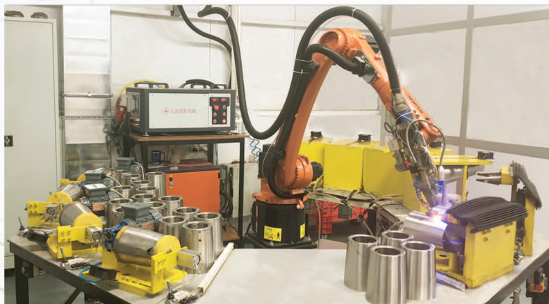
Laser Safety Room
