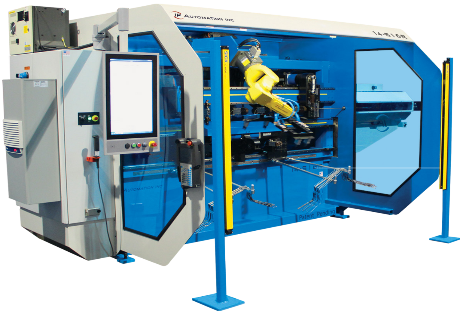
CNC MULTI-HEAD BENDING MACHINE FOR 3-DIMENSIONAL WIRE FORMS
